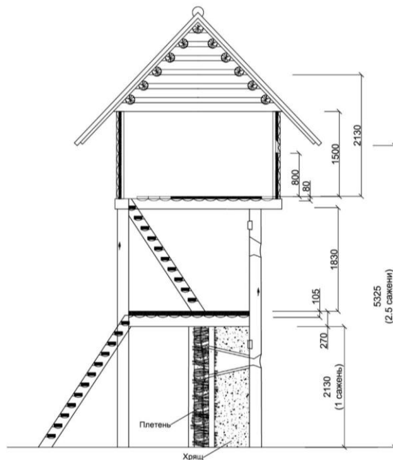
Fig. 9. Option number 3. The design of the wall with the “gorodnya” and “nagorodnya”. Author's reconstruction (Yarovoï B. P., Trukhin V. I.)
